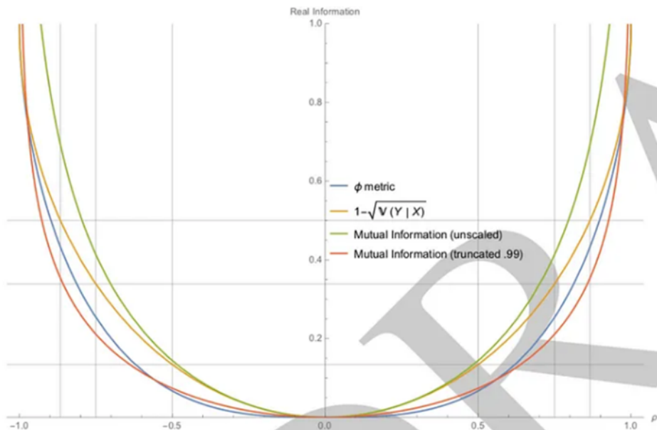
Fig. 6. Various rescaling methods, linearizing information and putting correlation in perspective.
