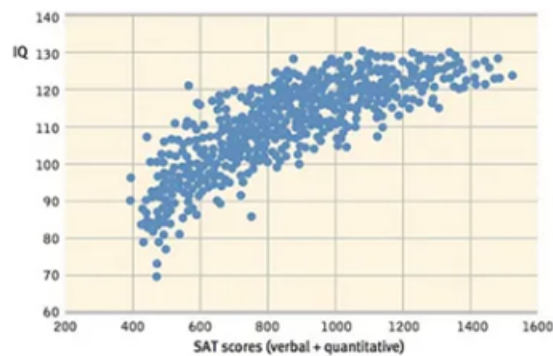
Figure 11.4 Close cousin: Aptitude and intelligence scores. A scatterplot shows the close correlation between intelligence scores and verbal and quantitative SAT scores. From Frey and Detterman, 2004. © 2010 by North Palatka
